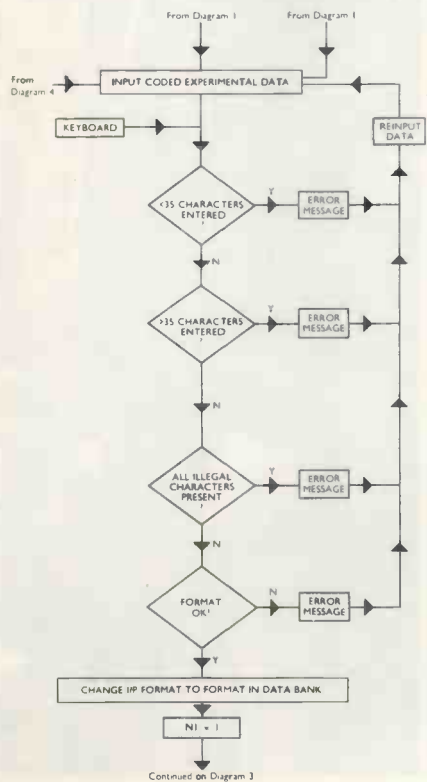
Diagram 2. Input data validation.
