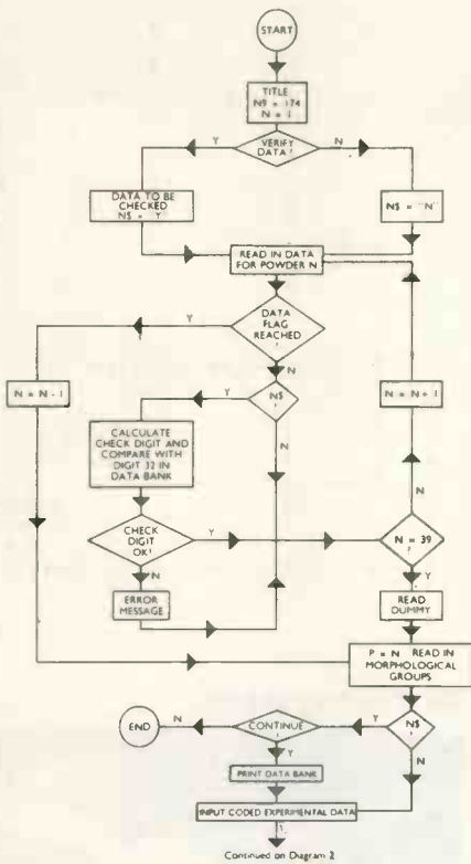
Diagram 1. Read data.
