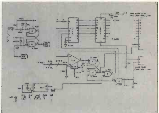
Figure 2. I/P interface board Pet 2.
